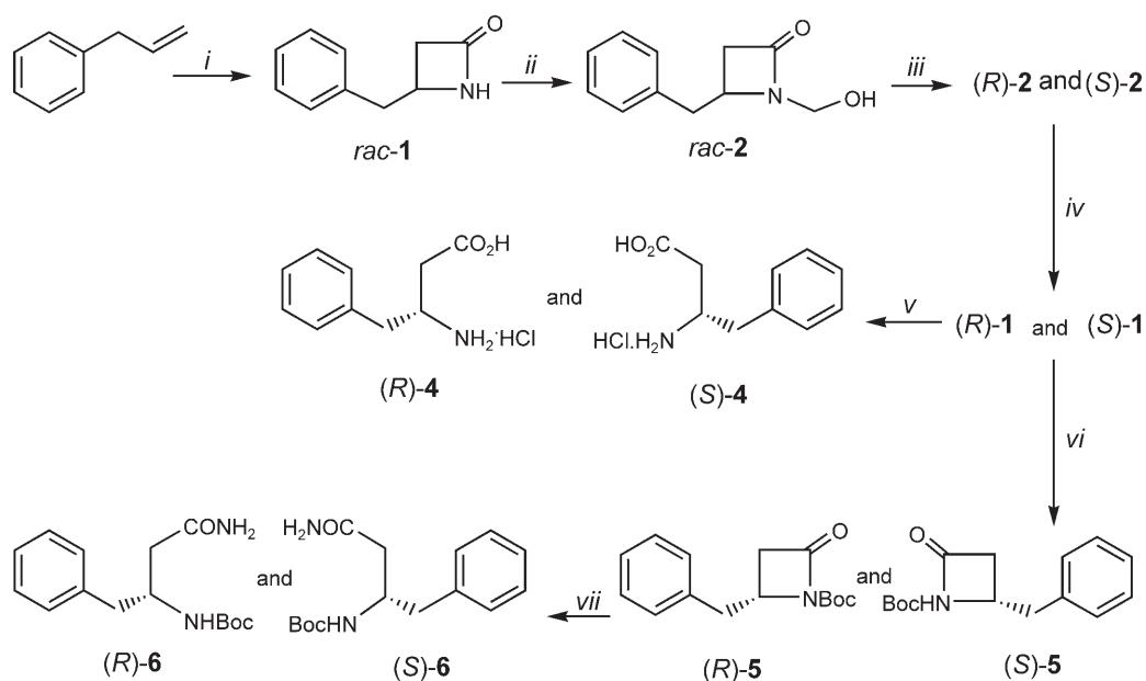
Scheme 1. i : CSI, CH 2 Cl 2 , 30 °C, then Na 2 SO 3 , K 2 CO 3 ; ii : paraformaldehyde, K 2 CO 3 , H 2 O, ultrasound, THF; iii : lipase-PS, first PrCO 2 CH=CH 2 then BuOH; iv : NH 4 OH, methanol; v : aqueous HCl (6 N); vi : (Boc) 2 O, NEt 3 , DMAP, CH 2 Cl 2 ; vii : 25% NH 3 in methanol.
