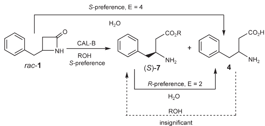
Scheme 2. CAL-B-catalyzed transformations in the reaction of rac -1 with alcohols and water.
