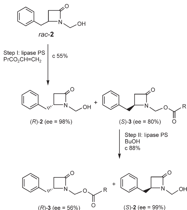
Scheme 5. Gram-scale preparation of ( R )- and ( S )-2.
