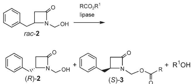
Scheme 3. Lipase PS-catalyzed acylation of rac -2.
