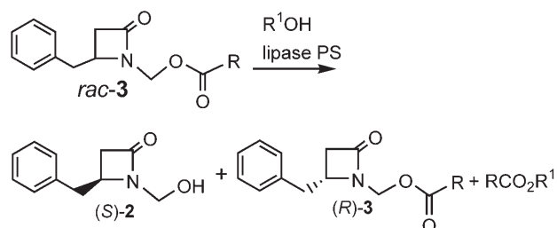
Scheme 4. Lipase PS-catalyzed alcoholysis of rac -3.
